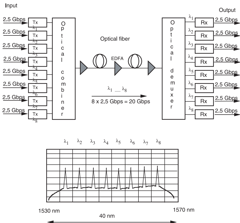
Figure 28.5 WDM with a capacity of 20 Gbps. (From A. A. Huurdeman, Guide to Telecommunications Transmission Systems , Artech House, Norwood, MA, 1997, Figure 2.21; with permission of Artech House Books.)
