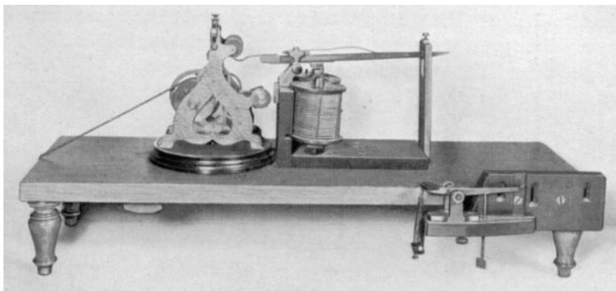
Figure 6.5 Morse telegraph as used for the Washington–Baltimore line. (Scanned from Ernst Feyereabend, Der Telegraph von Gauss und Weber , Reichspostministerium, Berlin, 1933, p. 85.)
