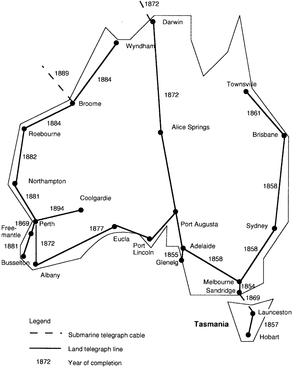
Figure 8.16 Major electrical telegraph lines of the nineteenth century in Australia.
