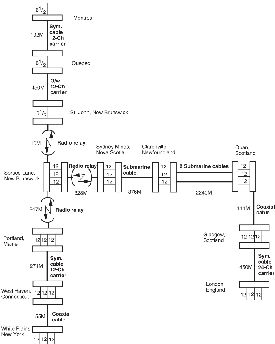
Figure 26.4 First transatlantic telephone cable, TAT-1.
