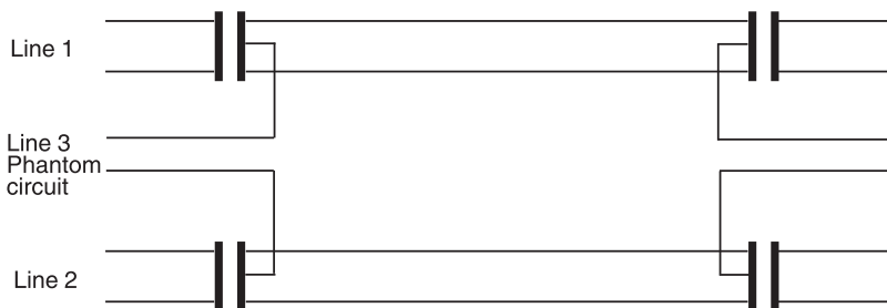
Figure 20.4 Phantom circuit arrangement.
