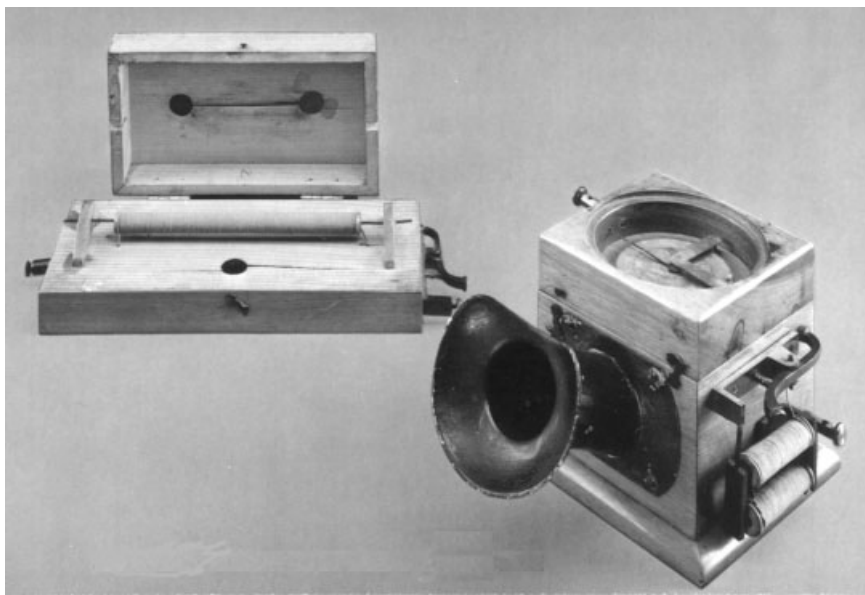
Figure 10.2 Telephon of Reis, 1863: left, the receiver; right, the transmitter. (Courtesy of Museum für Kommunikation, Frankfurt, Germany.) See insert for a color representation of this figure.
