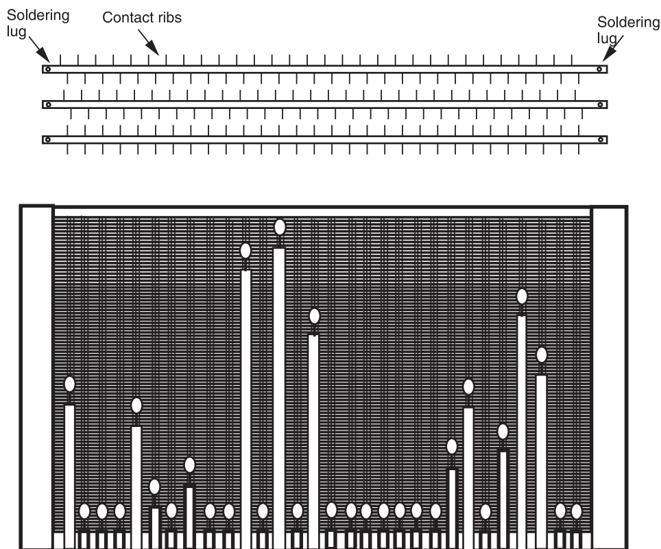
Figure 16.9 Panel system.
