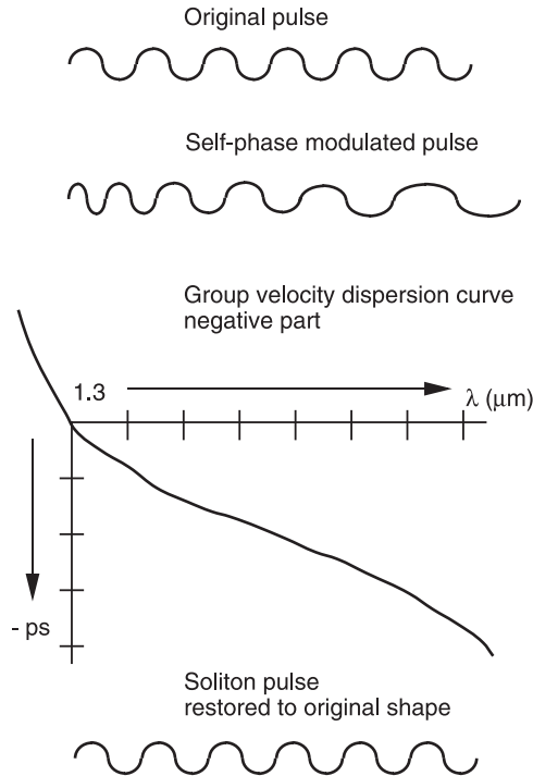
Figure 28.4 Soliton transmission. (From A. A. Huurdeman, Guide to Telecommunications Transmission Systems , Artech House, Norwood, MA, 1997, Figure 4.8; with permission of Artech House Books.)
