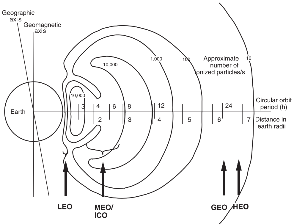
Figure 27.1 Satellite orbits. (After Robert A. Nelson, Satellite constellation geometry, Via Satellite , March 1995, p. 112. Originally from A. A. Huurdeman, Guide to Telecommunications Transmission Systems , Artech House, Norwood, MA, 1997, Figure 7.4; with permission of Artech House Books.)
