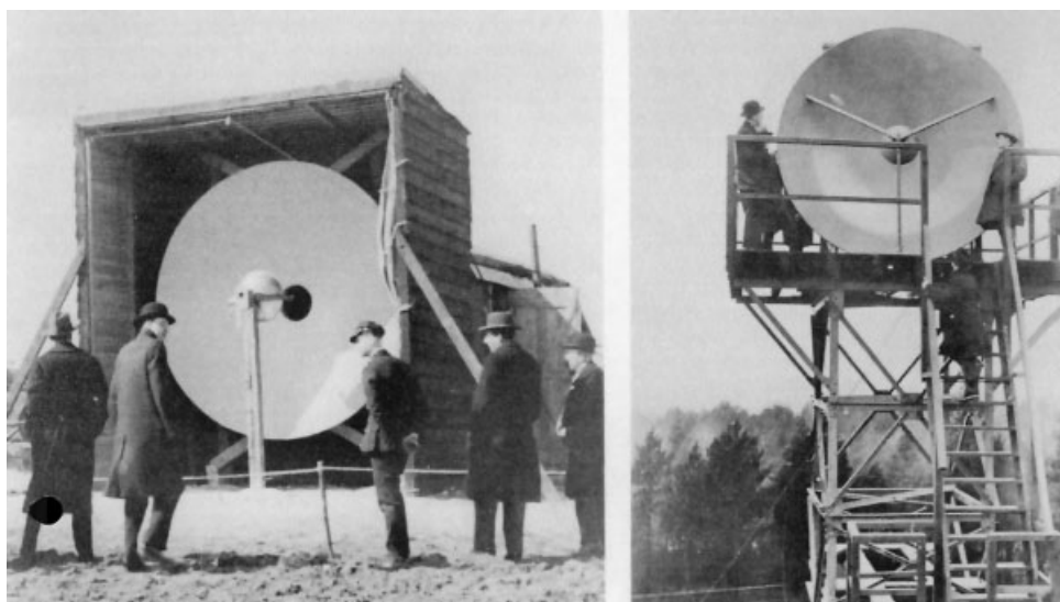
Figure 21.3 World's first experimental radio-relay terminals at both sides of the English Channel, 1931: left, at Calais; right, at Dover. (Scanned with permission of the ITU from Anthony R. Michaelis, From Semaphore to Satellite , International Telecommunication Union, Geneva, 1965, p. 163.)
